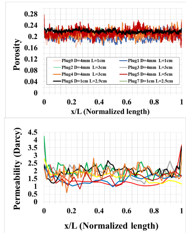
Fig. 1. Porosity and permeability profiles obtained via 3D image processing of the Bentheimer plugs used in this study and numerical simulation using segmented images on OpenFoam ® respectively. For porosity, the uncertainty on segmentation is estimated at \pm 0.4 p.u. and we must add +1 to 2 p.u. for the clay part.
