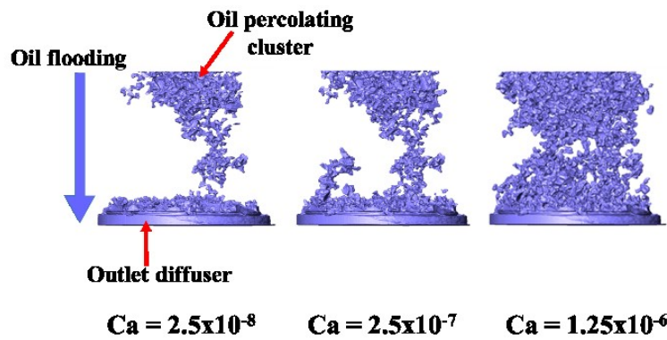
Fig. 9. Oil cluster spreading out and accumulating at the outlet during primary drainage of a Bentheimer plug (diameter = 4mm) at various rates. Magnification is the same in both directions and the diffuser is 4 mm diameter.
